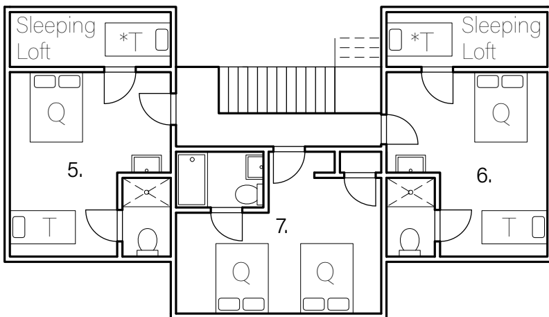
Second Floor
